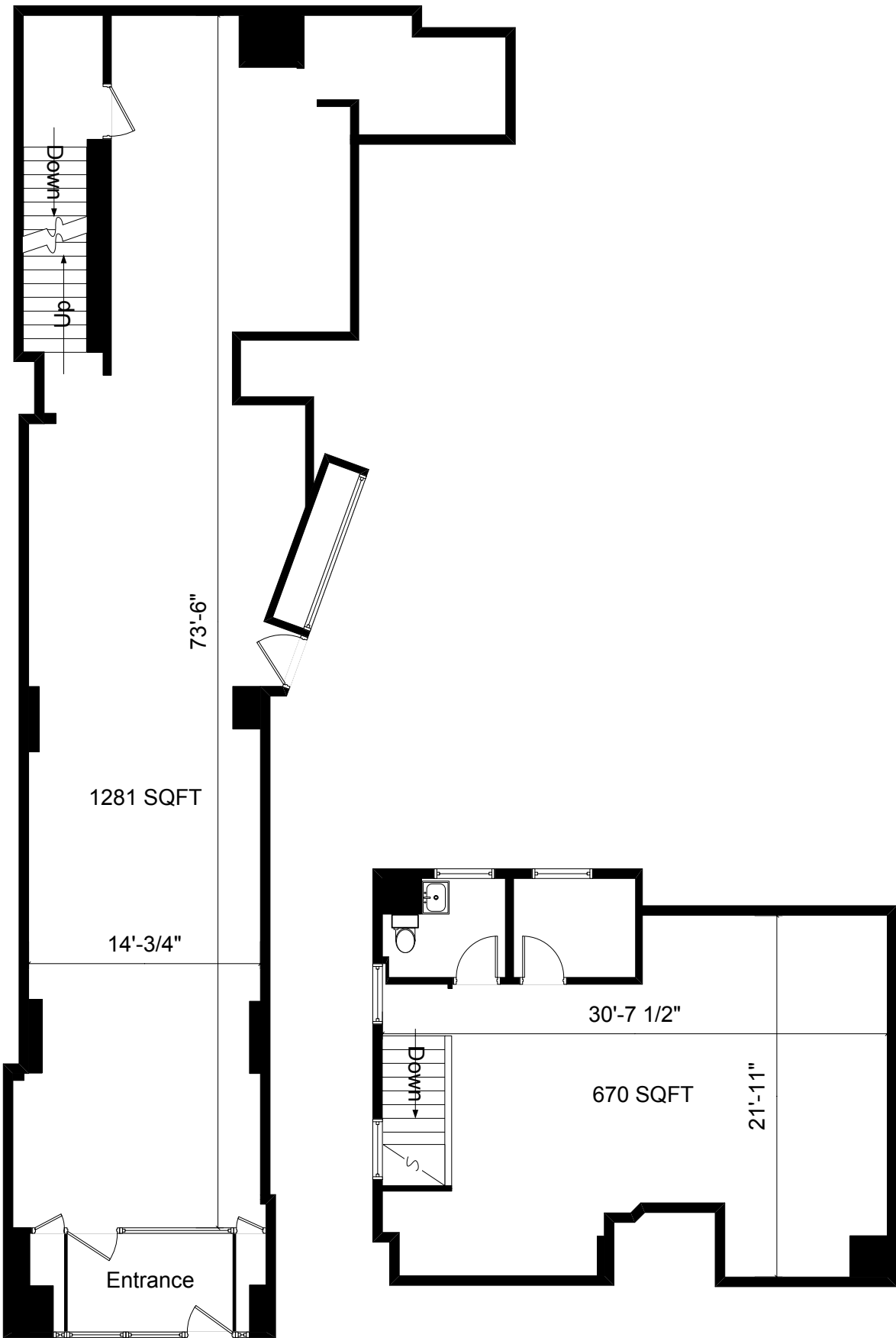
MAIN LEVEL
